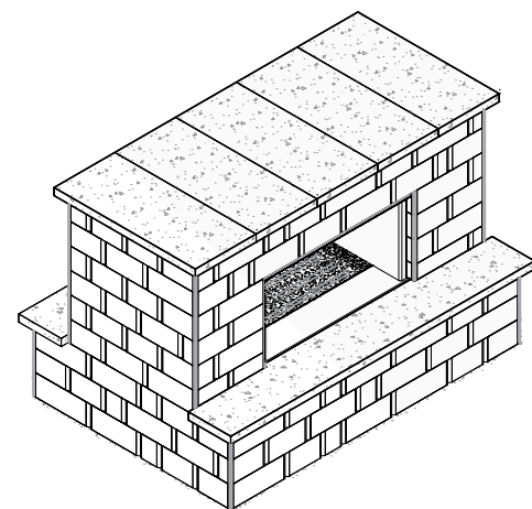
2-sided/2-hearth Fireplace
