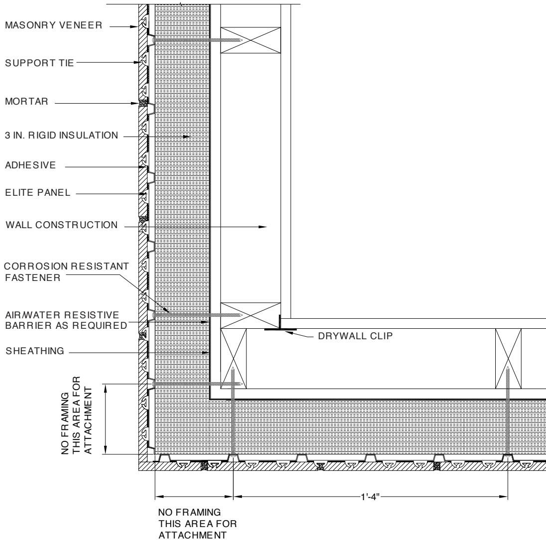
FIGURE C-2 – PLAN VIEW AT 2-STUD CORNER
