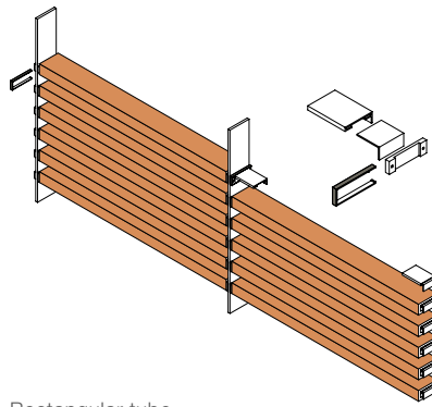
Rectangular tube
