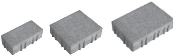
4x8 4" x 8" x 3 1/8"
