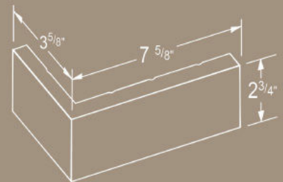
Queen Corner 2 3/4" x 3 5/8" x 7 5/8"
