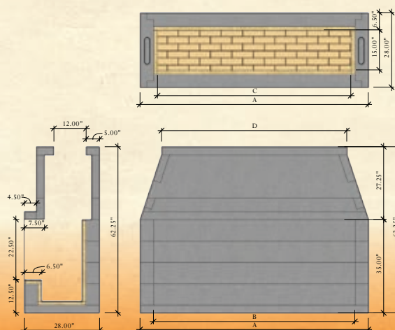
TROUGH LAYOUT
