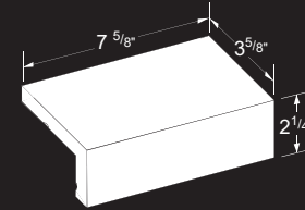
Modular Edge Cap 2 1/4" x 3 5/8" x 7 5/8" x 5/8"
