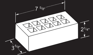
Modular Full Brick 2 1/4" x 7 5/8" x 3 5/8"
