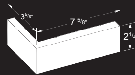
Modular Corner 2 1/4" x 3 5/8" x 7 5/8" x 5/8"
