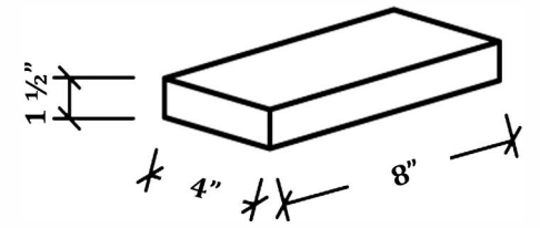
PUEBLO PLANT THICK SPLIT 4 x 8 PAVER
