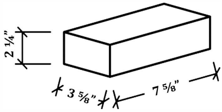
PUEBLO PLANT MODULAR PAVER
