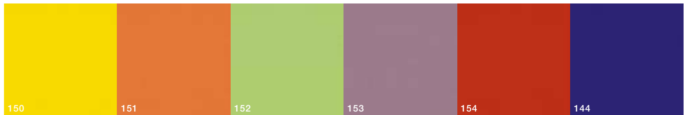
lemon-yellow H
