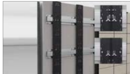
Fasten Omega profile with Al blind rivet (Art. no. 658) or A4 stainless steel screw (Art. no. 659) (Pay attention to fixed and sliding point)
