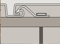
Hidden Fastener System
